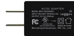
WALL CHARGER
